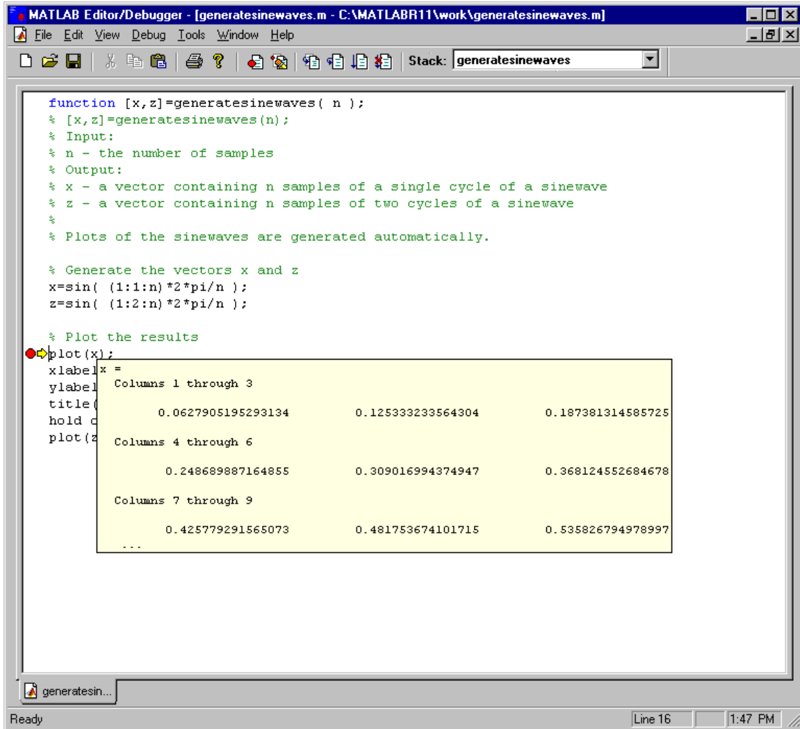
Figure 4 – An m-edit debugging session. Execution has halted at the breakpoint before the ‘plot’ command. The cursor is placed over the variable x which causes its contents to be displayed.
