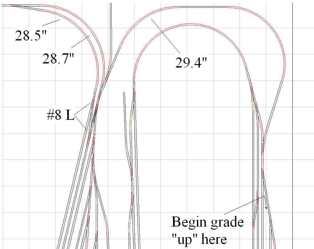
Track component detail showing exceptions to standard radius and turnout #
